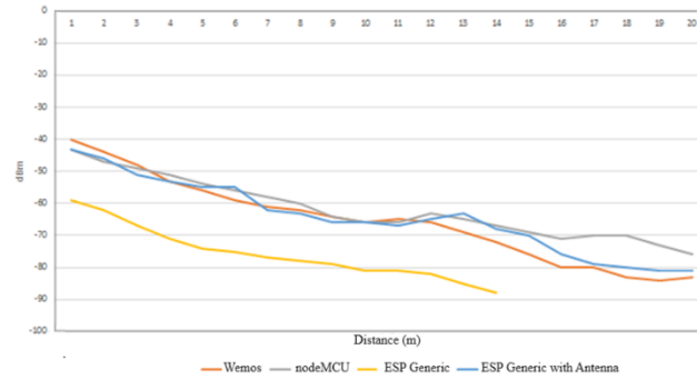
Fig. 2. Comparative graphic image of ESP8266 module signal gain
